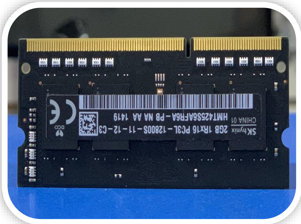
RR-DDR3L-010 Memoria RAM Laptop 2gb DDR3, 1333Mhz
